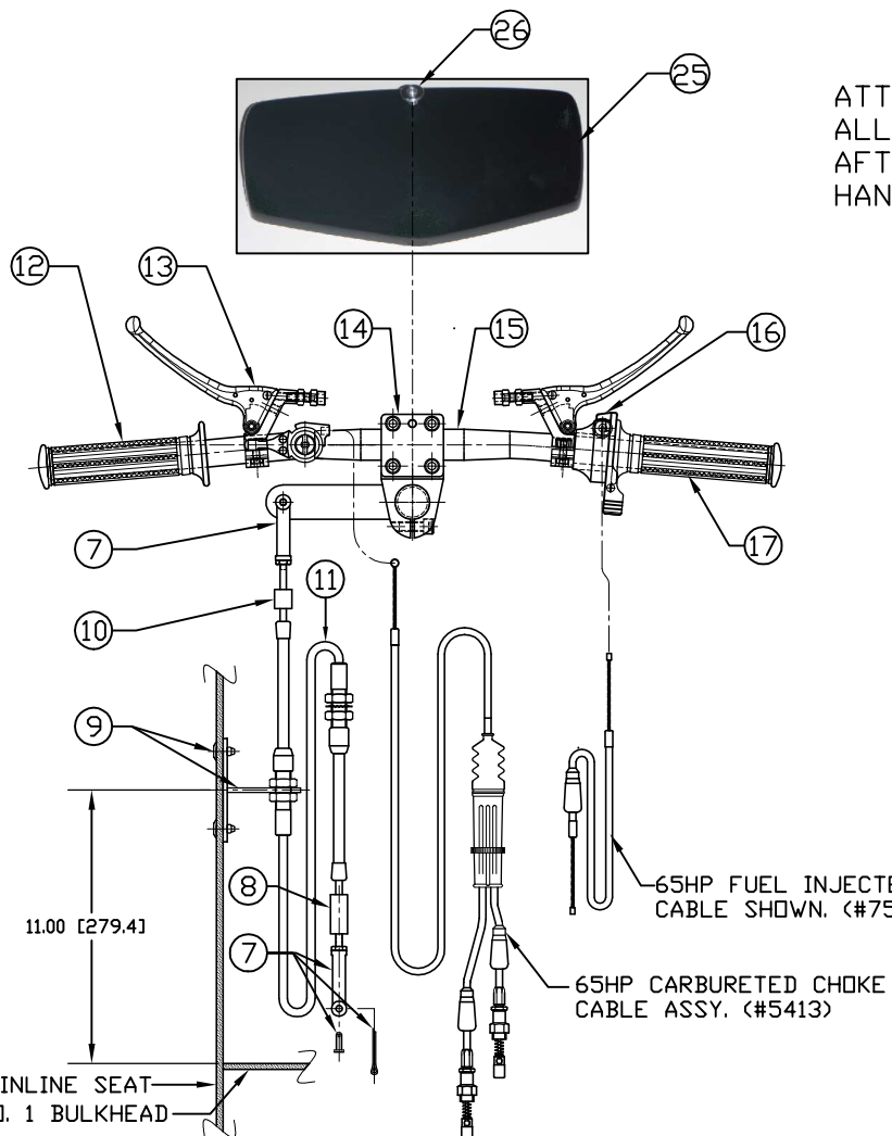
TOP VIEW
