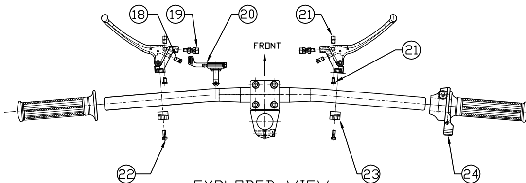
EXPLODED VIEW
