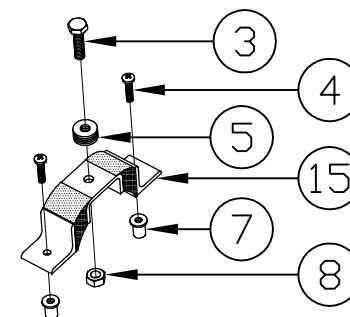
OLD STYLE EXHAUST MOUNT (DISCONTINUED Q3 2014)
